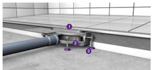
1 Channel cover 2 Drain body 3 Installation supports
