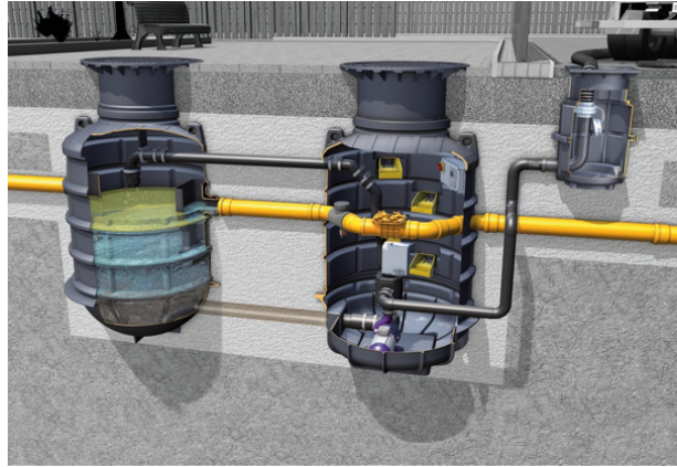
installation example grease separator EasyClean ground Auto Mix & Pump (Source: KESSEL)
