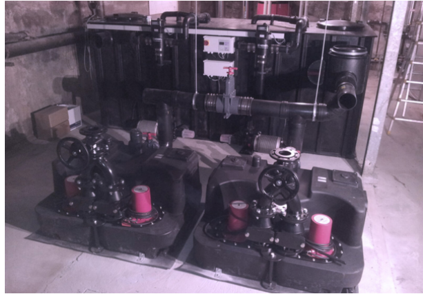
Installation situation "Zum Augustiner" (Source: KESSEL)
